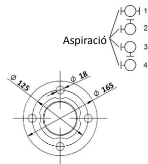
BRIDA ASP-IMP.
